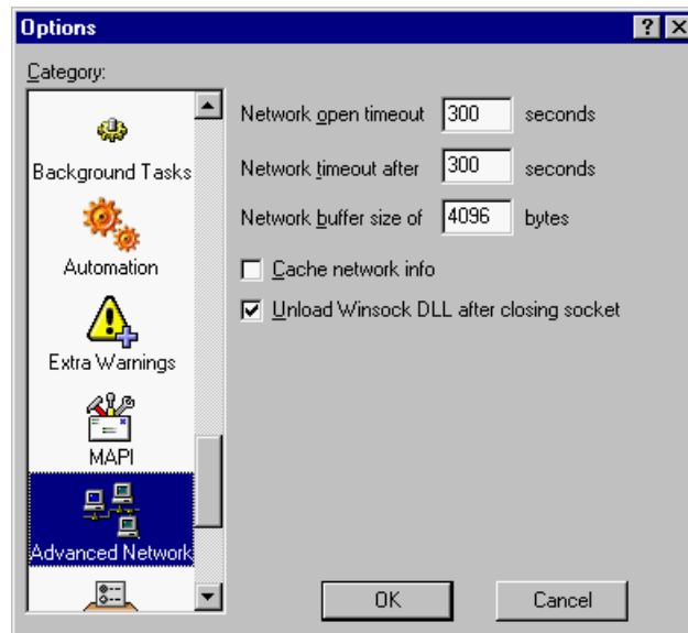
Advanced Network options window
