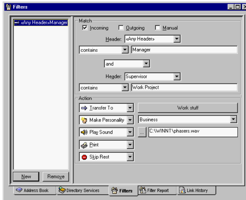
Filters window showing an example filter
