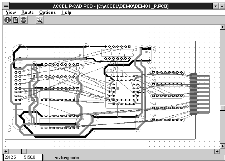
the menu and Toolbar offer autorouting options when ACCEL PRO Route is running
