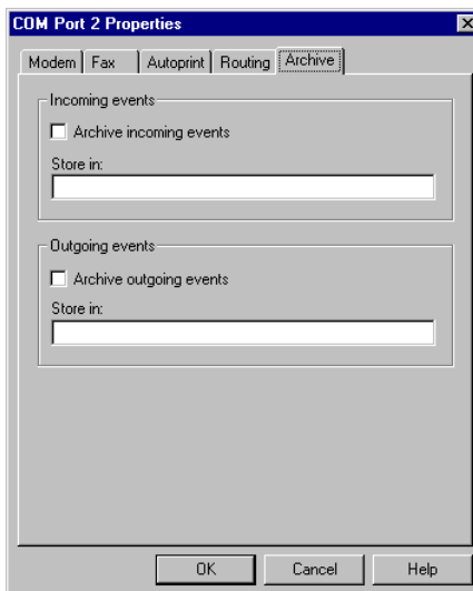
Archiving properties
