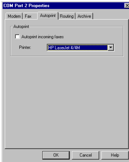
Autoprint properties
