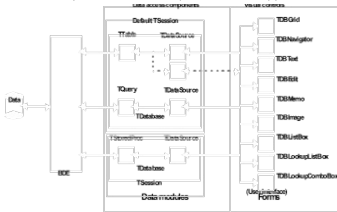
Relationship of database components in an application
