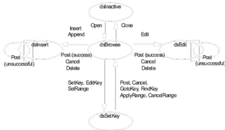
Relationship of Browse to other dataset states
