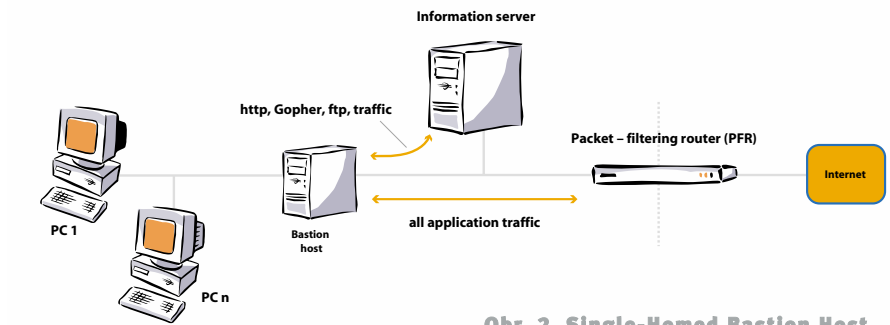
Obr. 2. Single-Homed Bastion Host
