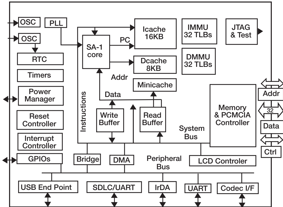
SA-1110 Block Diagram
